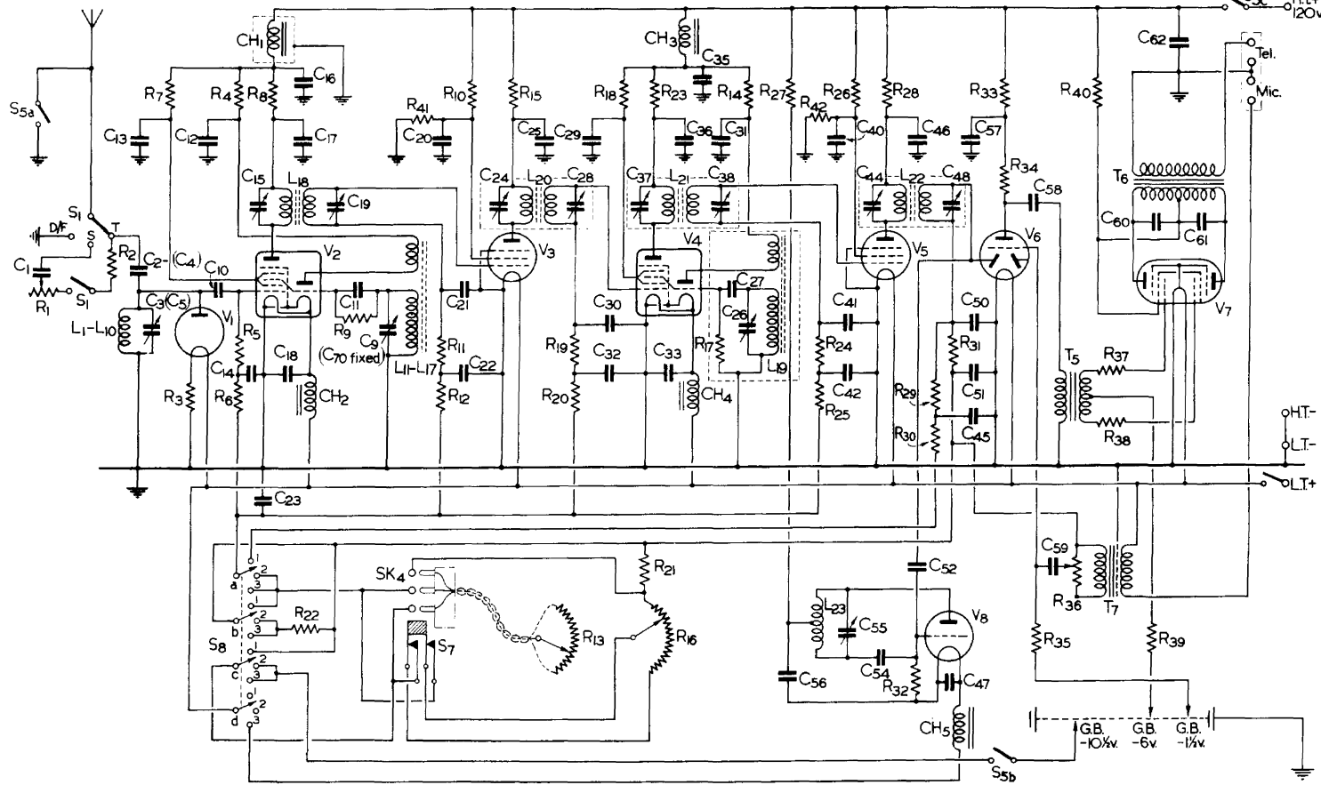
R1116 SIMPLIFIED CIRCUIT DIAGRAM
